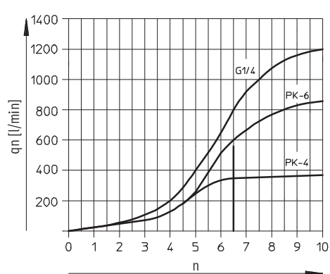
Rosca G1/4
