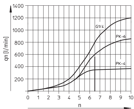
Rosca G1/4
